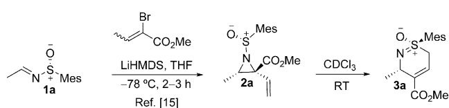
Scheme 1. Unprecedented rearrangement of aziridines leading to sulfoximines. HMDS = hexamethyldisilazide, Mes = 2,4,6-trimethylphenyl, THF = tetrahydrofuran.
